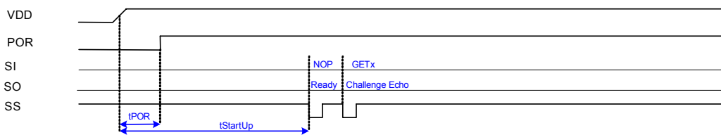
Figure 21 – Start-up sequence, basic scenario, timing diagram
