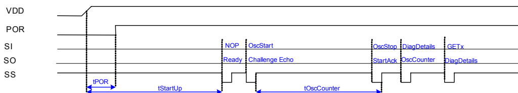
Figure 22 – Start-up sequence, safety critical scenario, timing diagram
