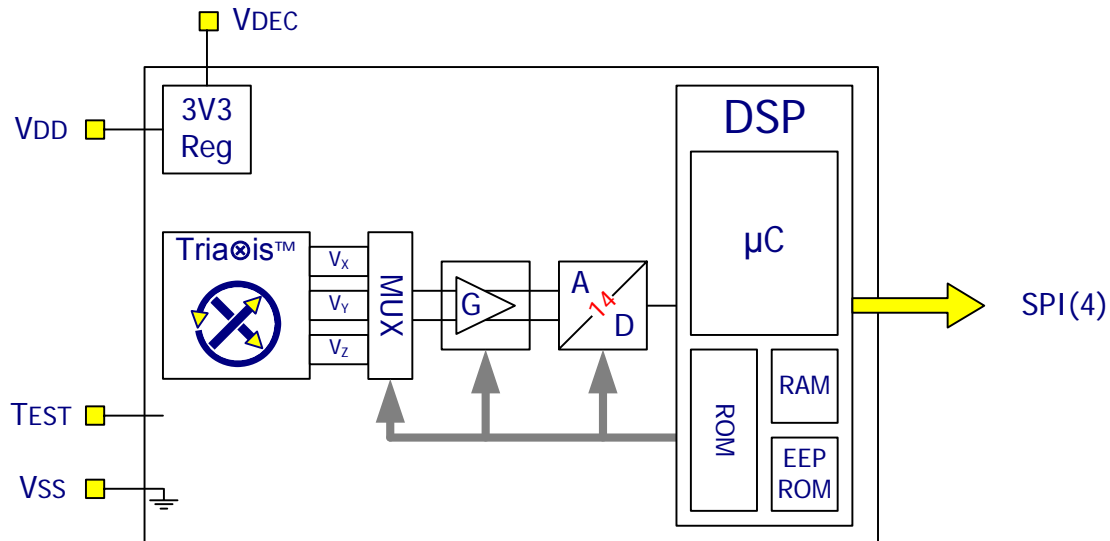
Figure 1 – Block Diagram
