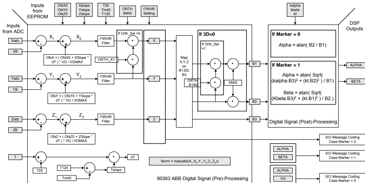
Figure 27 – Block Diagram of Signal Processing – Function model
