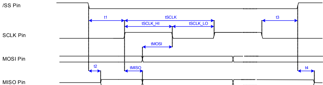
Figure 2 – Serial Interface Timing Diagram
