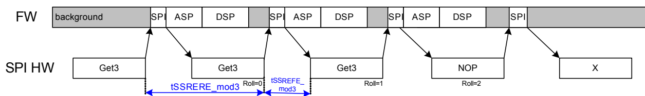
Figure 9 – Trigger mode 3
