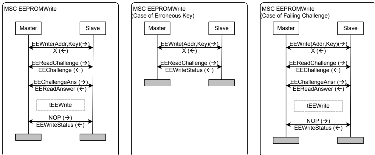
Figure 19 – MSCs EEPROMWrite
