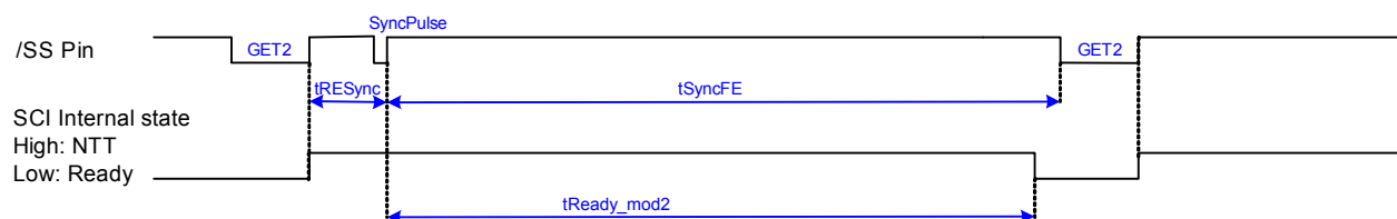
Figure 12 – Trigger mode 2 timing diagram
