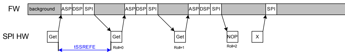
Figure 4 – Trigger mode 1
