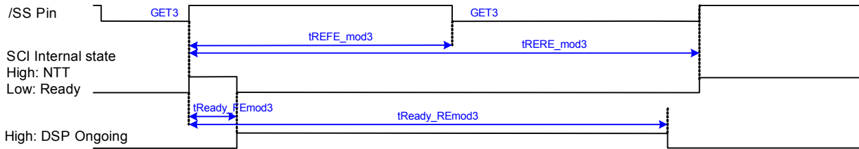
Figure 13 – Trigger mode 3 timing diagram
